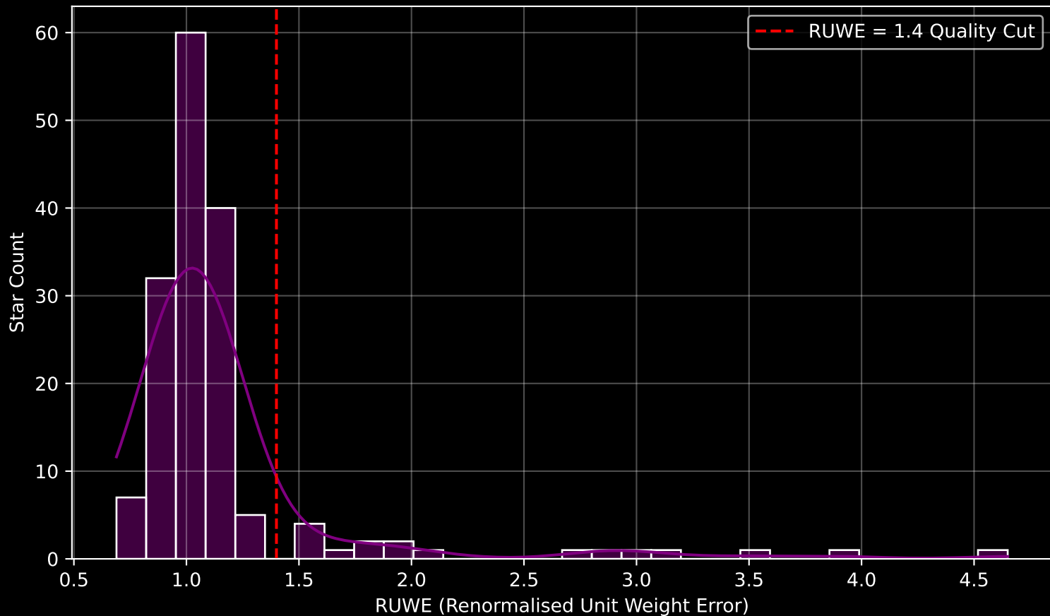
GALAH DR4 Field [7138] RUWE Distribution (n= 161)
