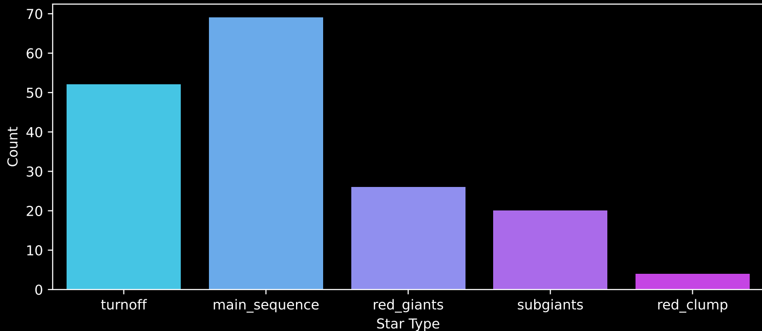
GALAH DR4 Field: [7138] Count plot of Star Type
