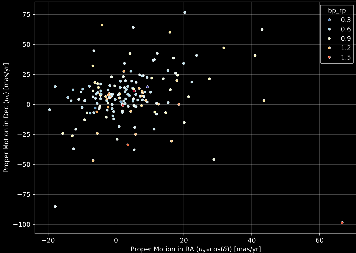
GALAH DR4 Field: [7138] Proper Motion Diagram (n= 171)
