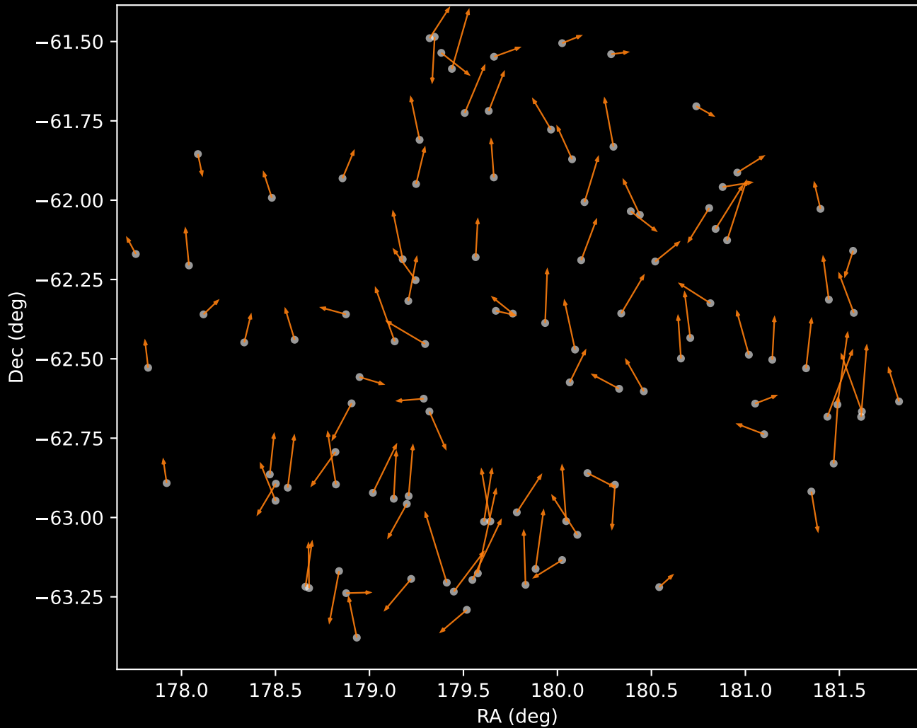
GALAH DR4 Cluster 2 Proper Motion Vectors (n=106)
